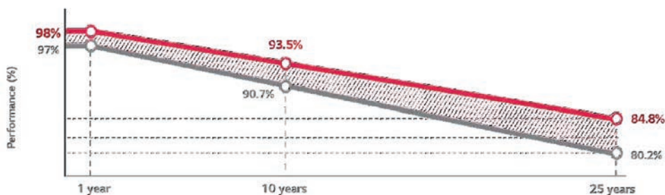
Annual Degradation
